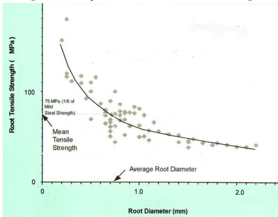
Fig.2 Relationship between root diameter and its tensile strength
