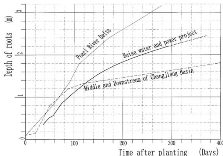
Fig. 1 Relationship between root depth and days after planting in spring and summer in South China. The data of the Middle and Lower reaches of Yangtze River were provided by the Traffic Department of Zhejiang Province, and all other data by the Guangzhou City Vetiver Grass Industry Science and Technology Co. Ltd.
